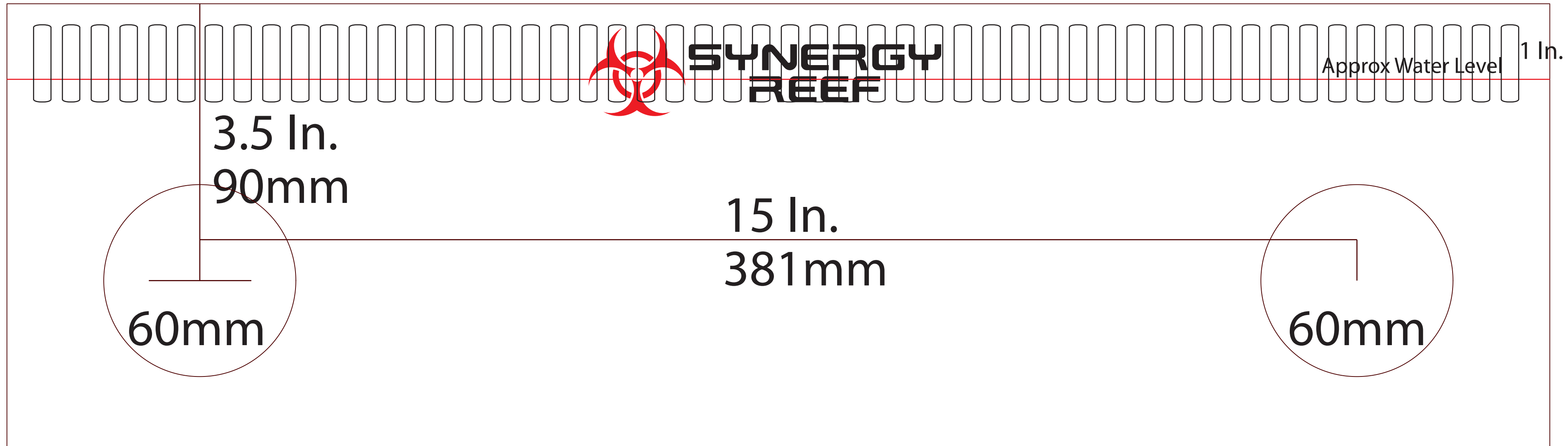
20" Synergy Reef Overflow Drilling Template
